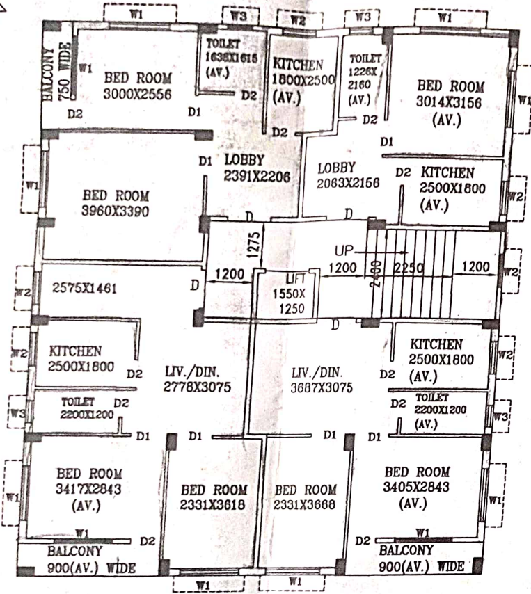
1ST & 2ND FLOOR PLAN SCALE 1:100
