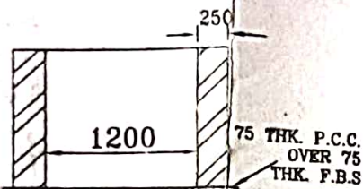
DETAIL SECTION OF VAT SCALE 1:50
