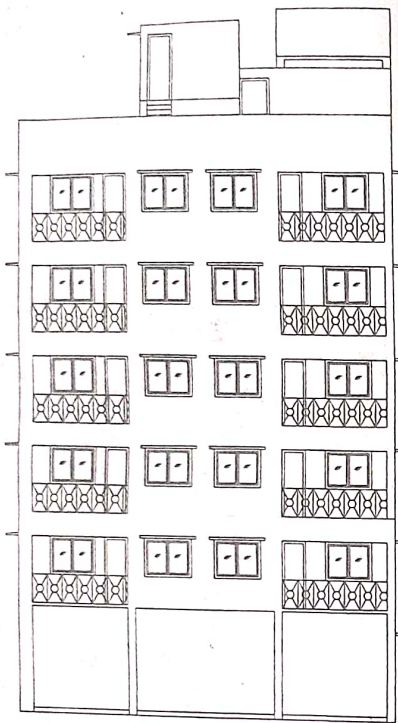
FRONT ELEVATION SCALE : 1:100
