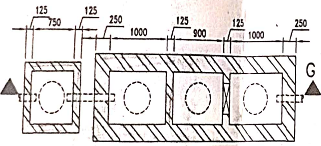
DETAILS OF SEPTIC TANK & CHLORINATION TANK SCALE - 1:50
