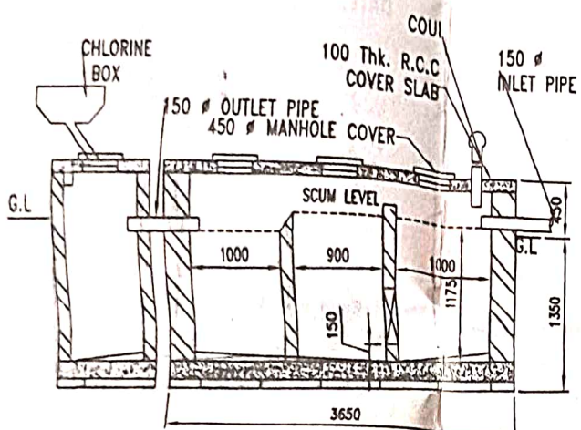
LONG. SECTION OF SEPTIC TANK & CH. PIT ON G-H SCALE 1:50
