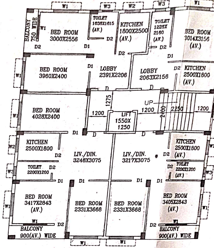
3RD 4TH & 5TH FLOOR PLAN SCALE 1:100
